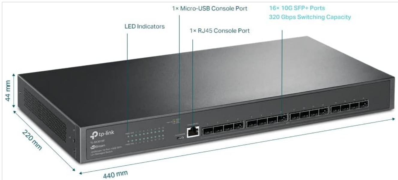
Figure 2: Angled view of the TL-SX3016F switch, highlighting 16 10G SFP+ Ports, 1 Micro-USB Console Port, 1 RJ45 Console Port, LED Indicators, and overall dimensions (440 mm x 220 mm x 44 mm).
