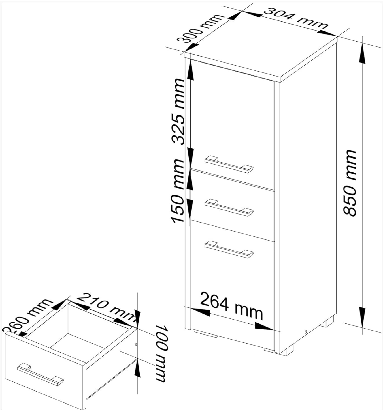
Image 2.1: Technical drawing illustrating the dimensions of the AKORD Bathroom Cabinet 85 2D1SZ, including overall height, width, depth, and internal drawer measurements.
