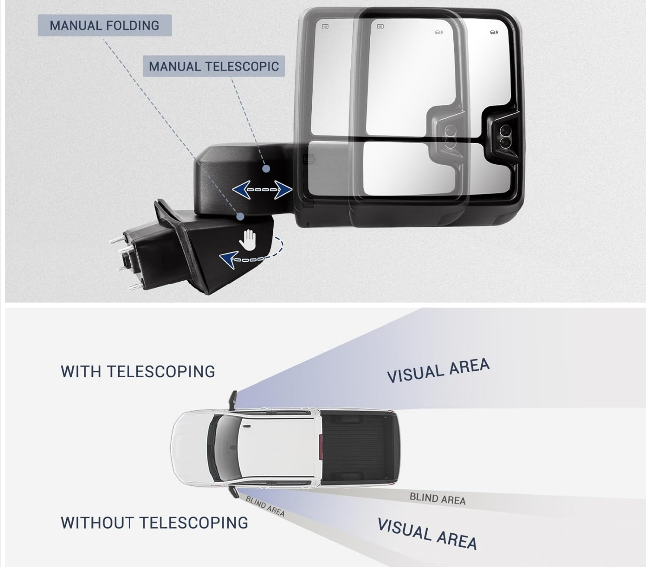
Figure 8: Manual Telescoping and Folding Mechanism
