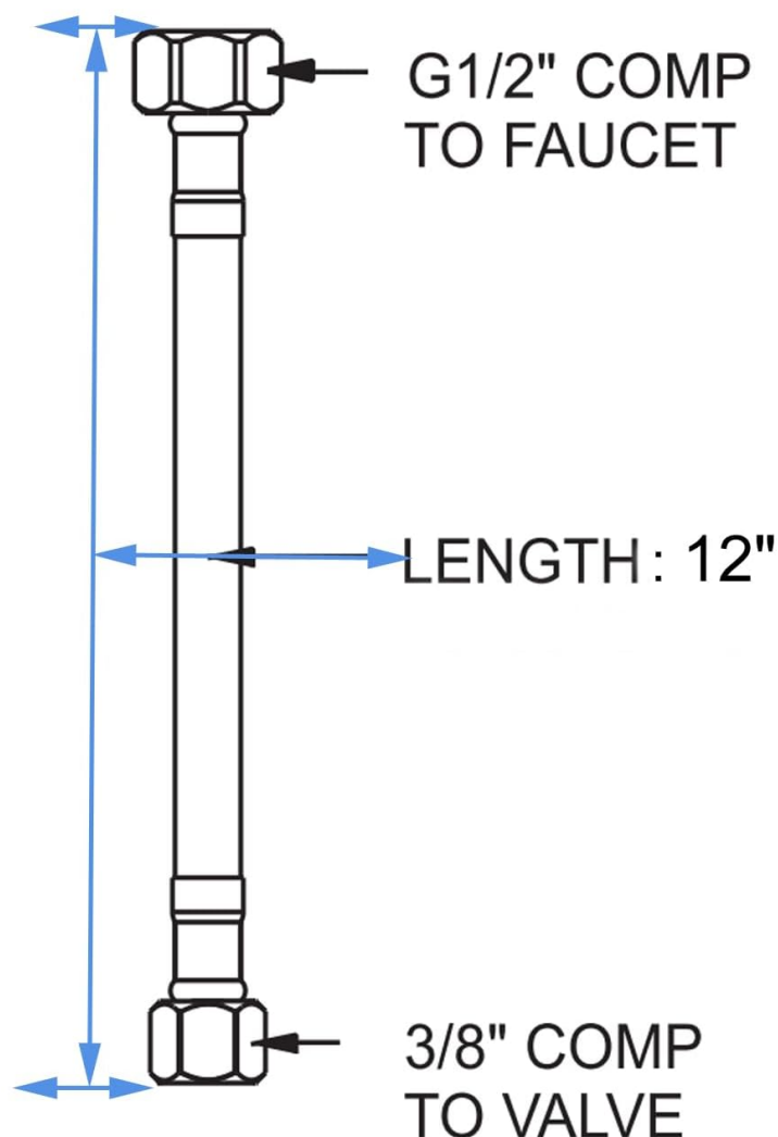
Image: A technical diagram showing the 12-inch length of the supply line, with the 3/8-inch compression end connecting to the valve and the 1/2-inch compression end connecting to the faucet.
