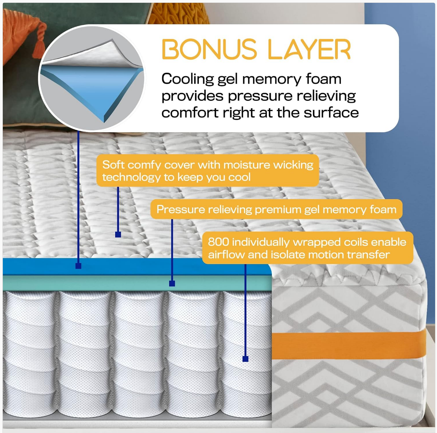
Figure 3.1: Cross-section diagram detailing the mattress layers and their functions.
