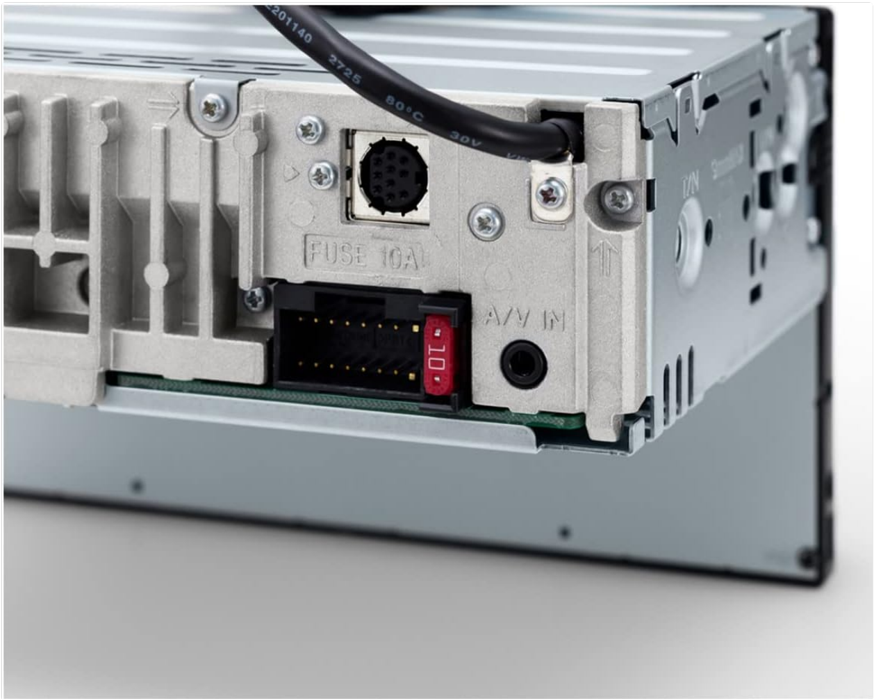
Image: A detailed view of the rear A/V input jack and the 10A fuse on the XAV-AX3200 unit, highlighting these specific connection points.
