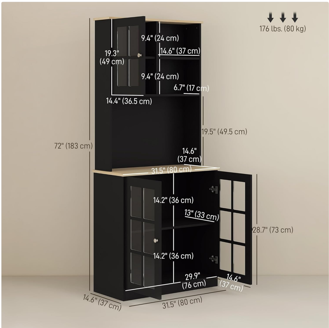
Figure 2: Detailed dimensions of the HOMCOM Kitchen Pantry. This diagram illustrates the height, width, and depth measurements of various sections, including shelves and the microwave stand area, in both inches and centimeters.
