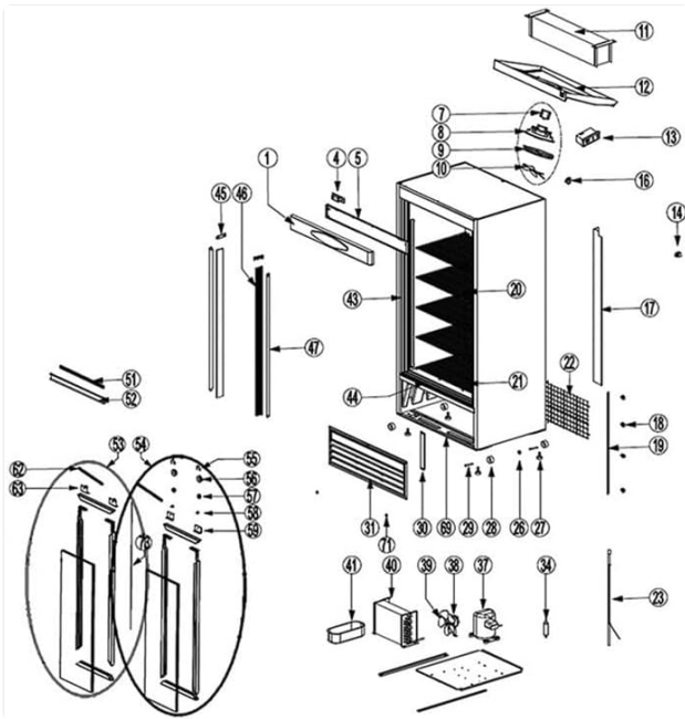
Figure 4: Exploded view diagram illustrating various internal and external components of the refrigerator for service and identification purposes.
