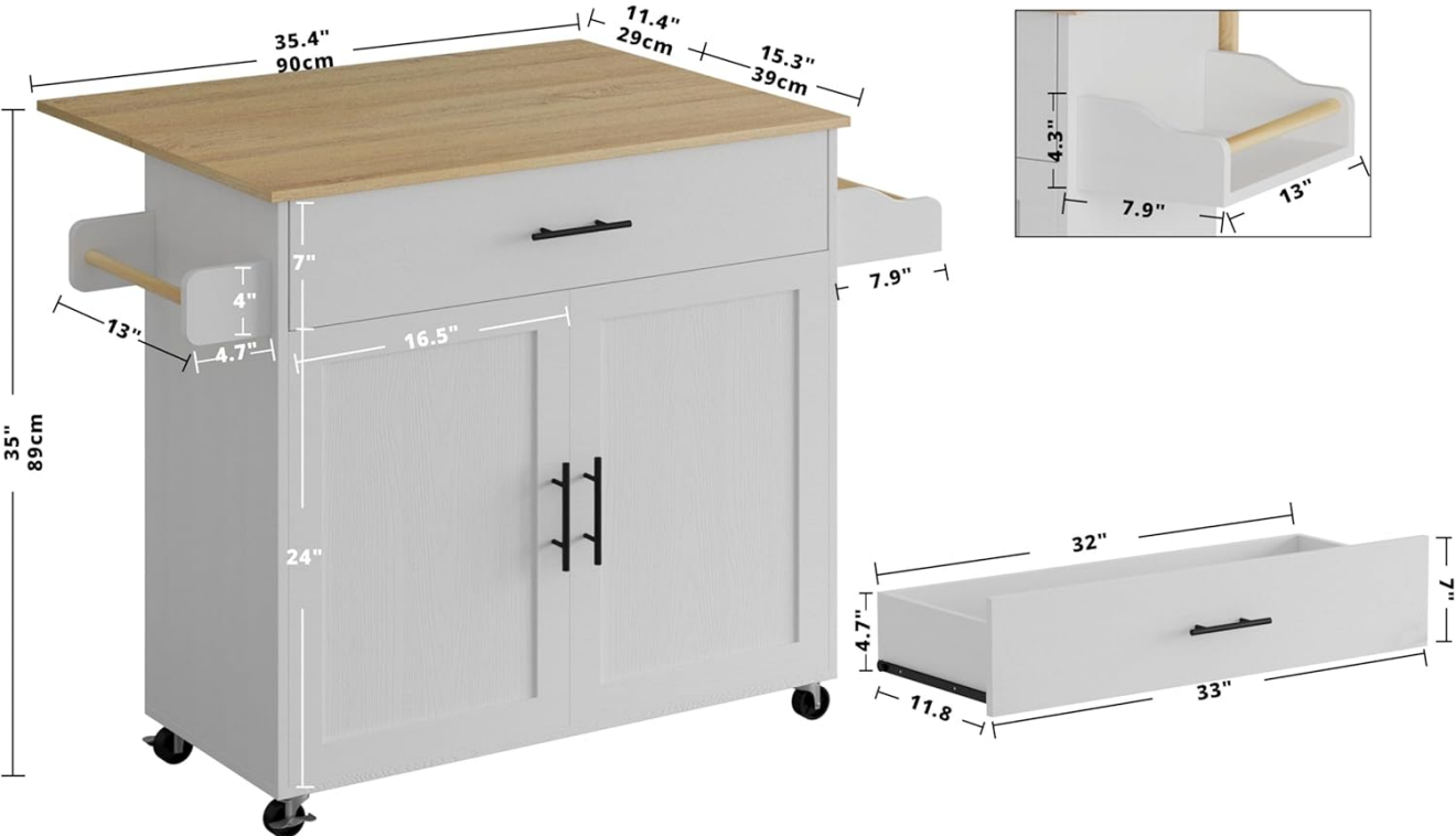
Figure 1: Overall Dimensions of the Kitchen Island.
