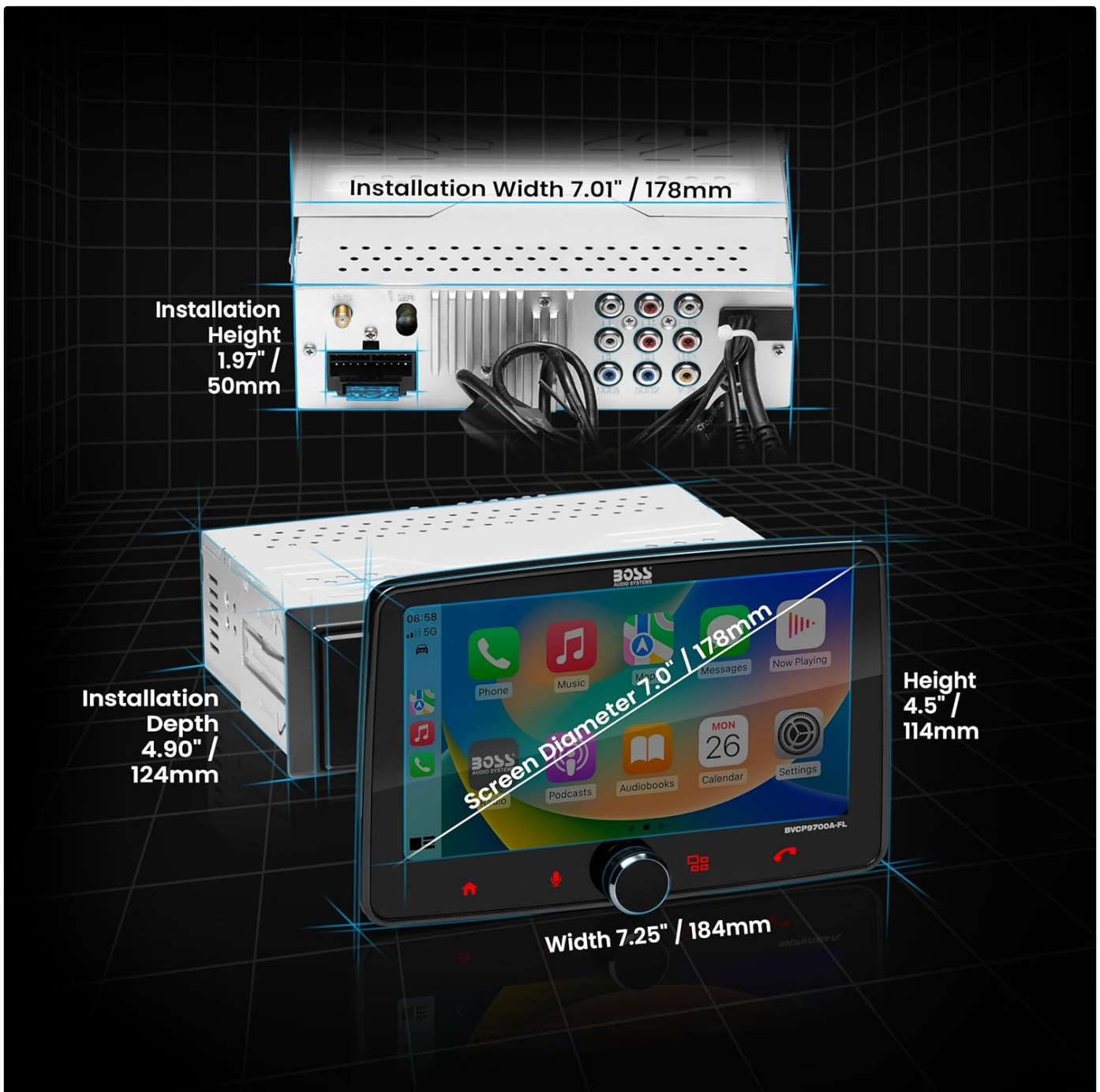
Figure 4.2: Detailed installation dimensions for the BVCP9700A-FL.
