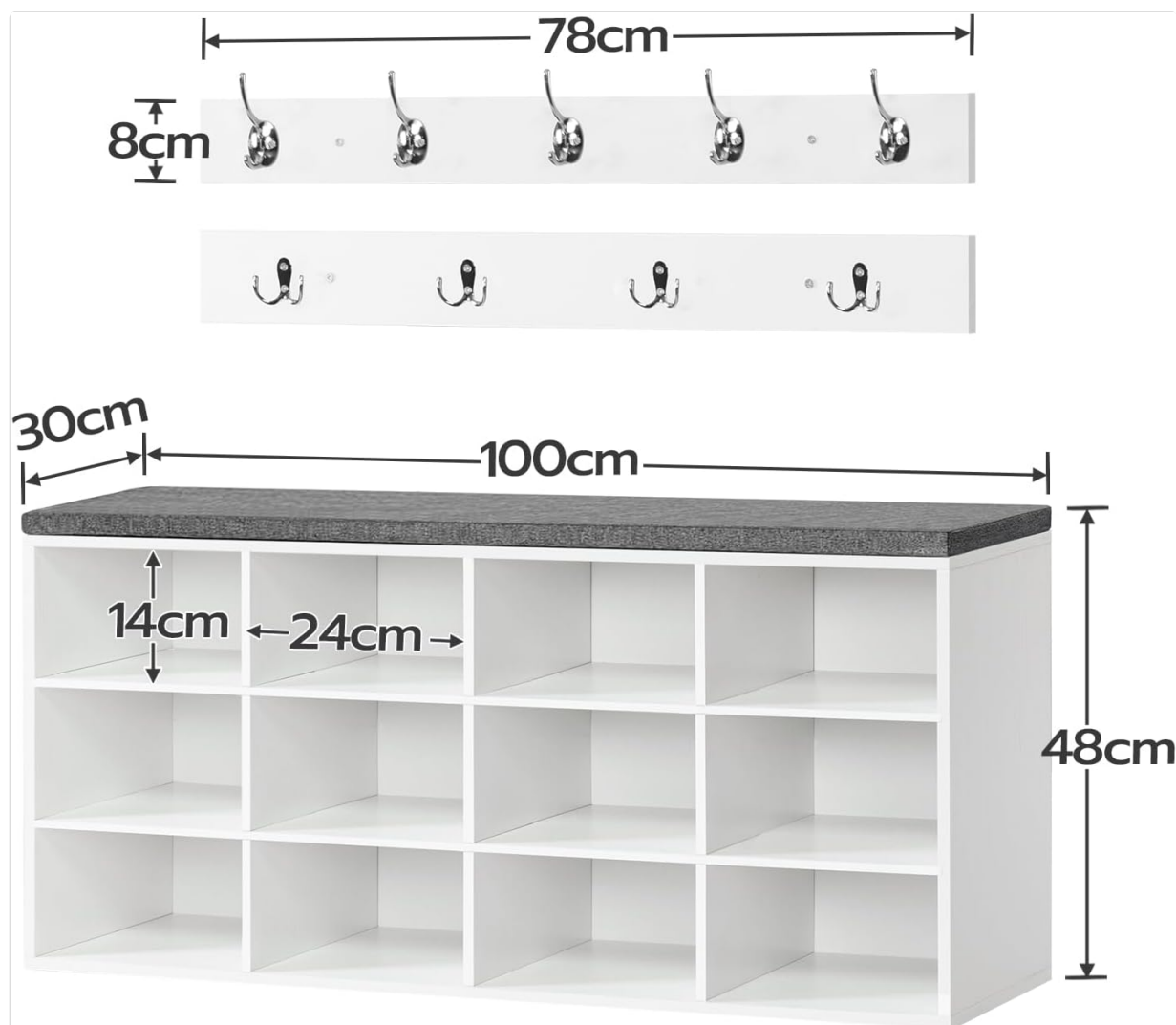
Image: Product dimensions for the shoe bench (100cm L x 30cm W x 48cm H) and coat rack (78cm L x 8cm H).
