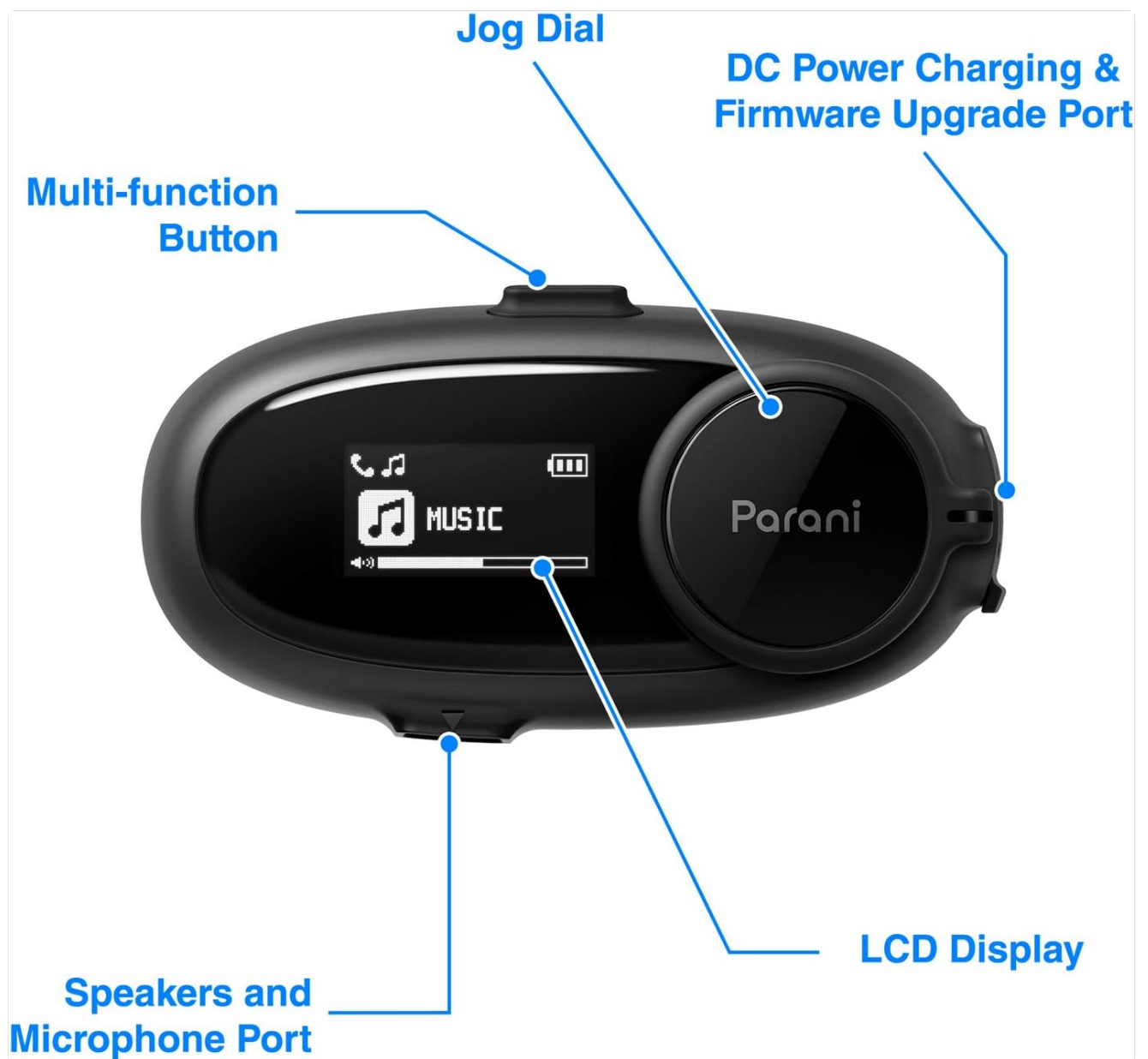
Figure 2.1: Parani M10 complete kit showing the main unit, wired microphone, and speakers.
