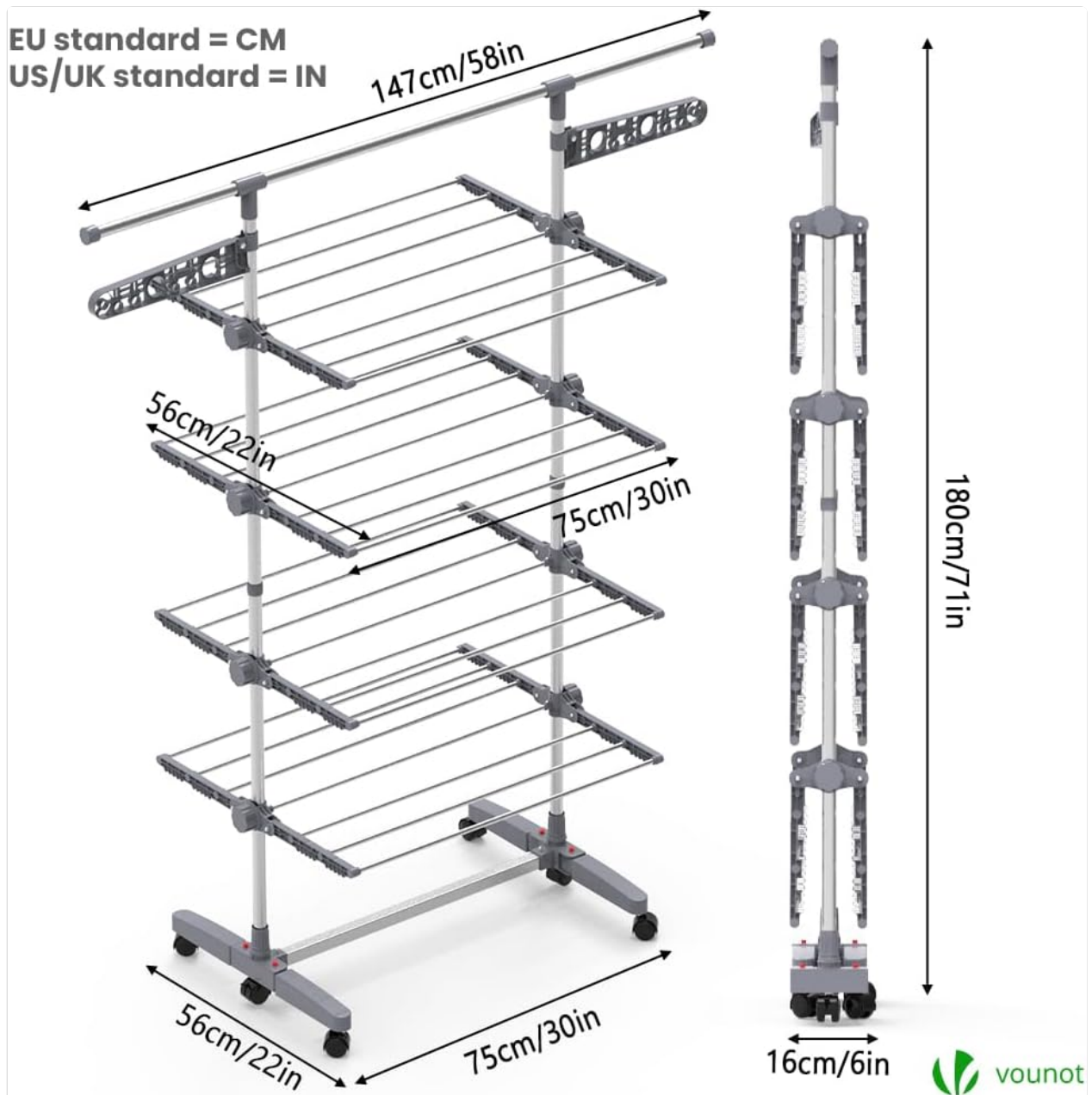
Figure 6: Dimensions of the drying rack in both unfolded and folded states.
