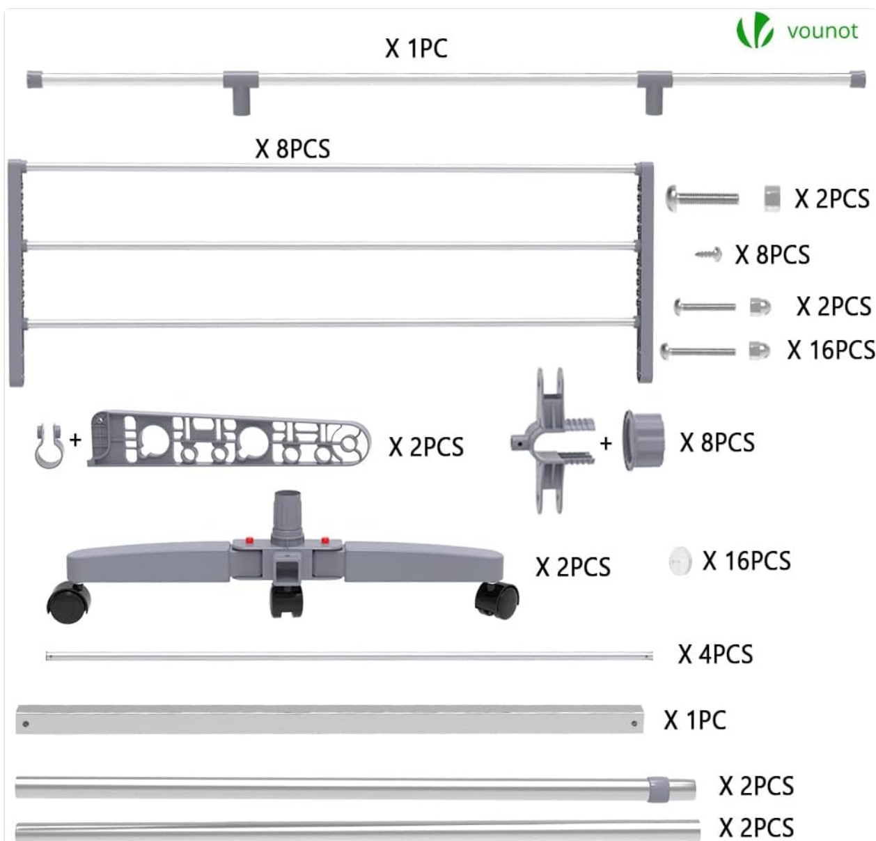
Figure 2: Exploded view of all parts included in the package.
