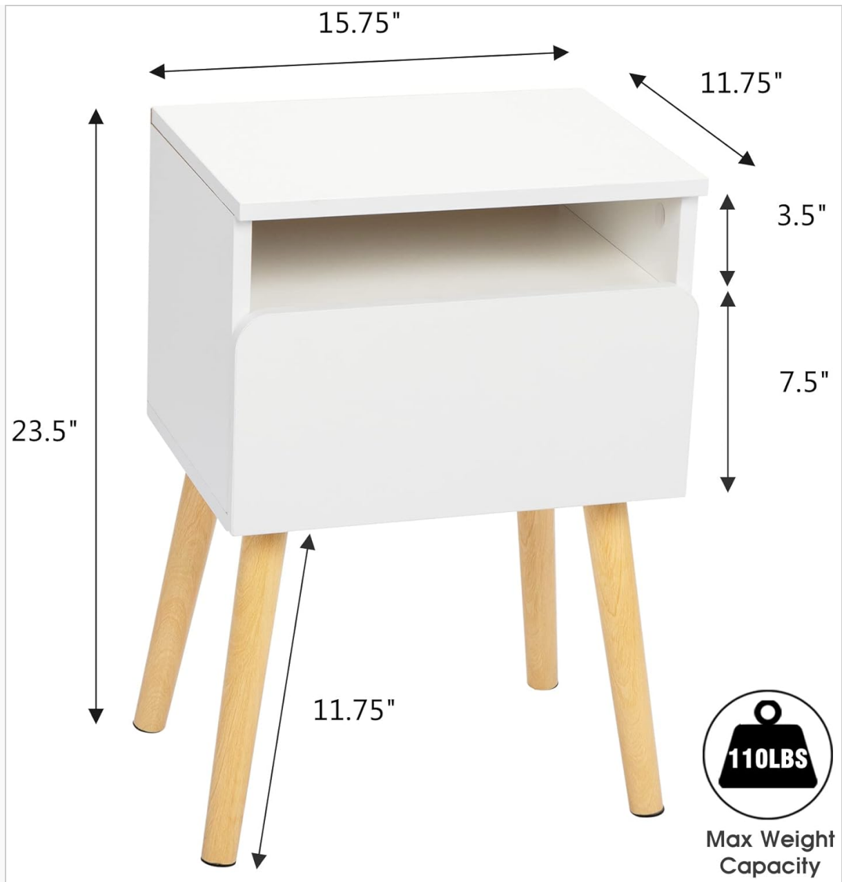
Image: Dimensional diagram and maximum weight capacity of the nightstand.
