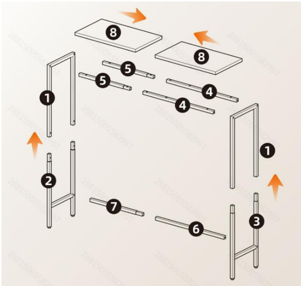
Image: Exploded view of the console table components, showing numbered parts for assembly.
