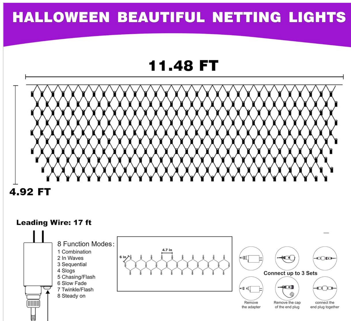
Figure 1: Net Light Dimensions and Connection Diagram
