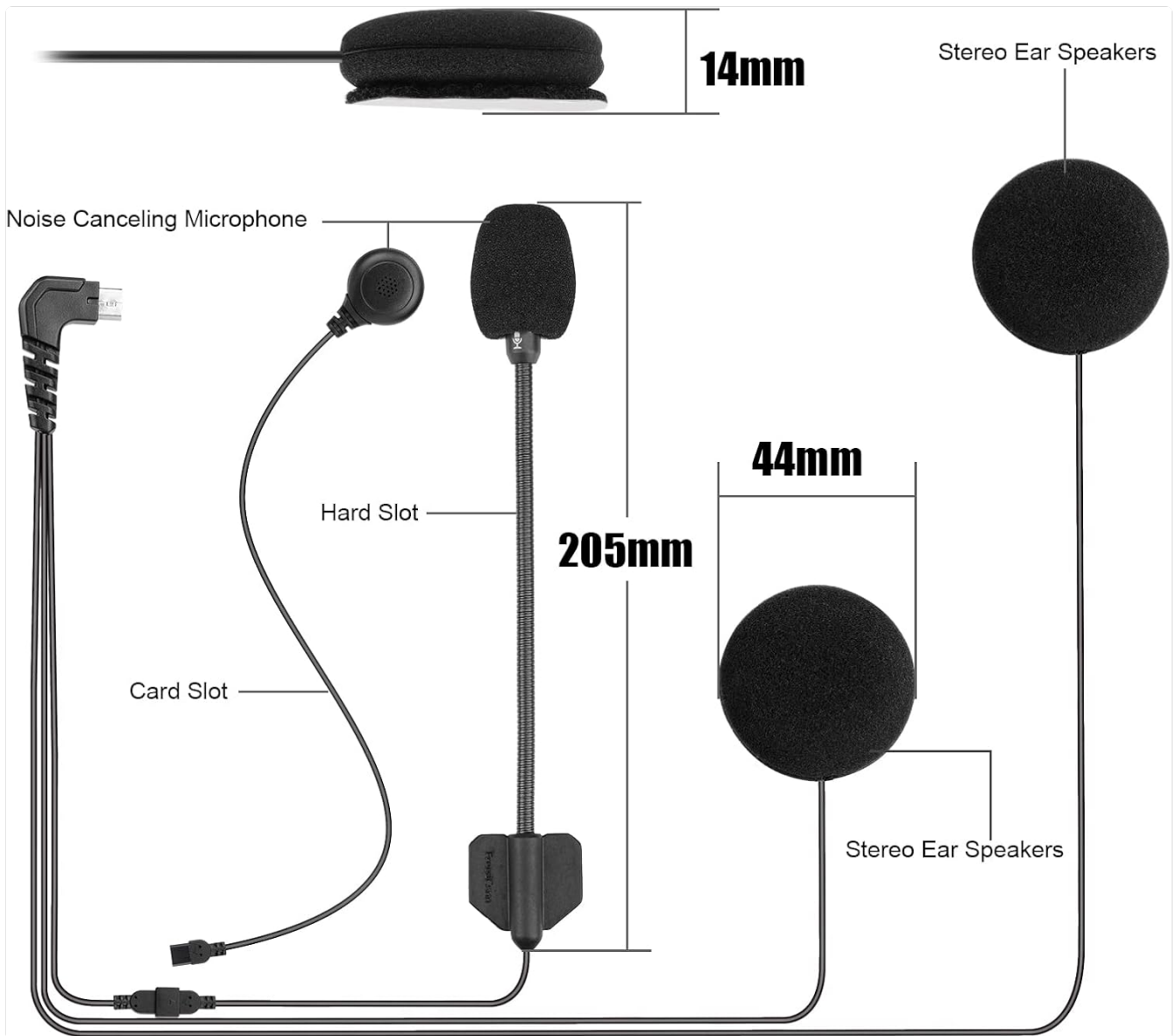
Image: Diagram showing the dimensions and components of the microphone and stereo ear speakers for installation.
