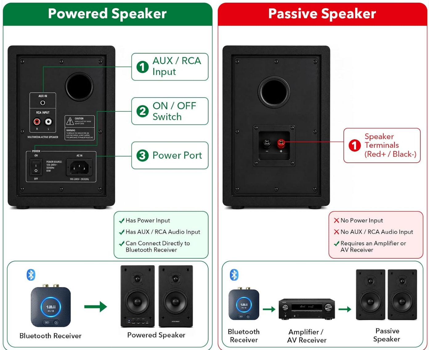
Figure 5: Connection methods for powered and passive speakers.
