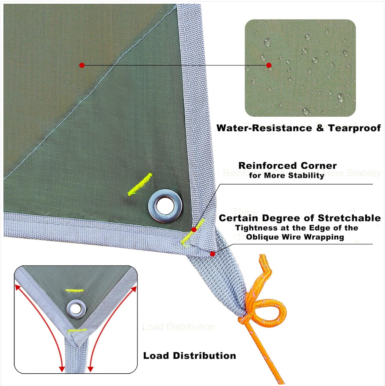
Image: Detail of the tarp's water-resistant and tearproof fabric with a reinforced corner for stability.
