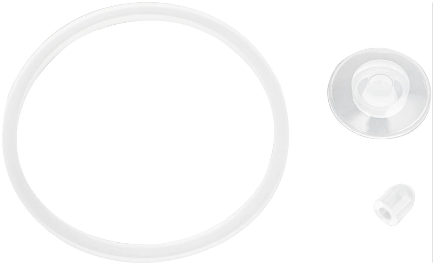
Figure 2.1: Overview of the Super Sparrow Replacement Sealing Parts. This kit typically includes a large silicone O-ring, a mouth seal, and an air hole plug.
