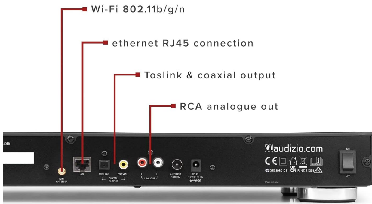
Image: Audizio Trento unit with remote control, showing approximate dimensions of 260mm length and 62mm height.
