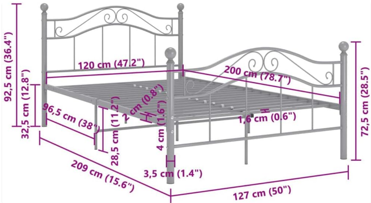
Image 8.1: Detailed dimensions of the bed frame.
