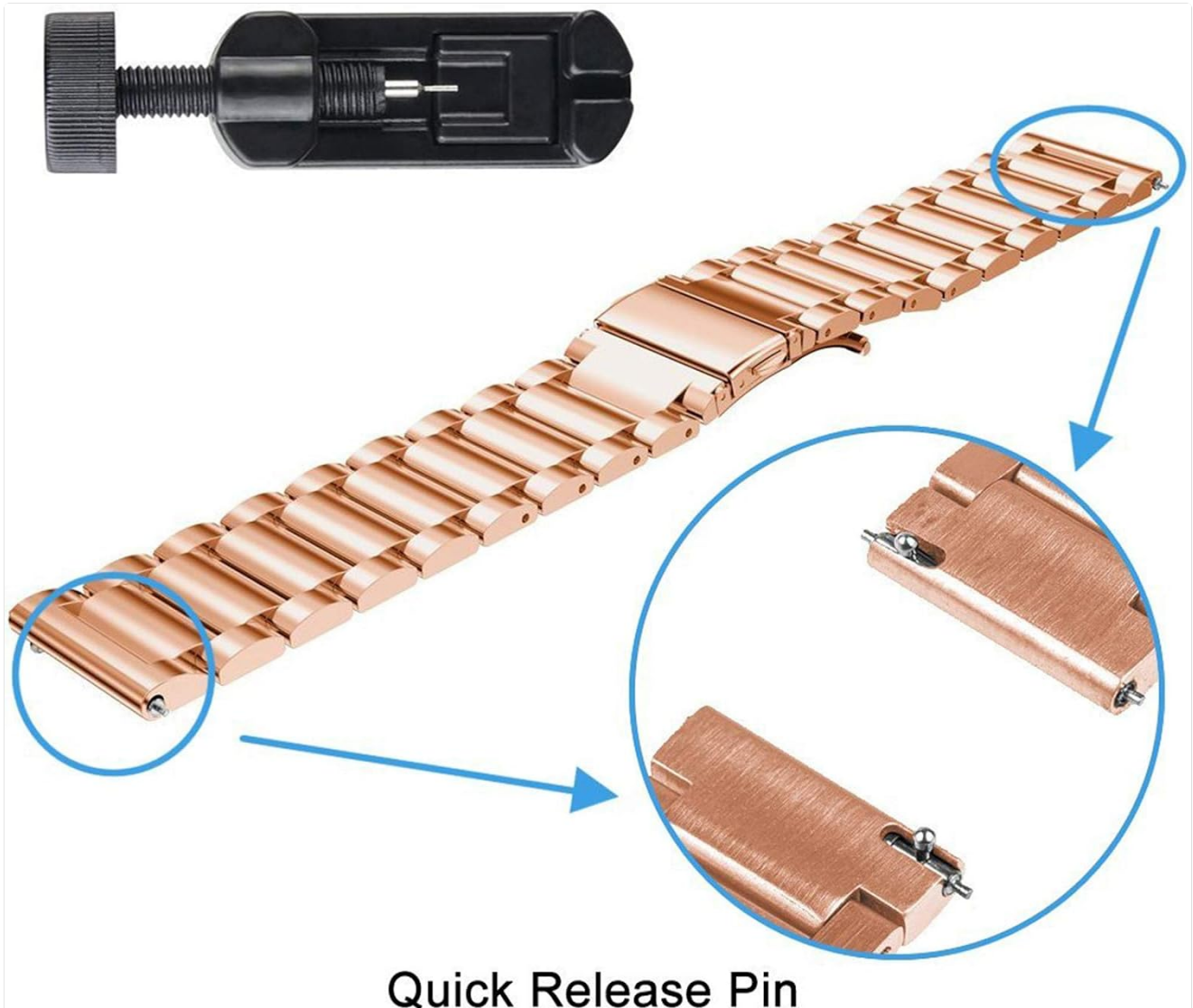
Image 2.1: A close-up view illustrating the quick-release pin mechanism on the watch band, designed for easy attachment and detachment.
