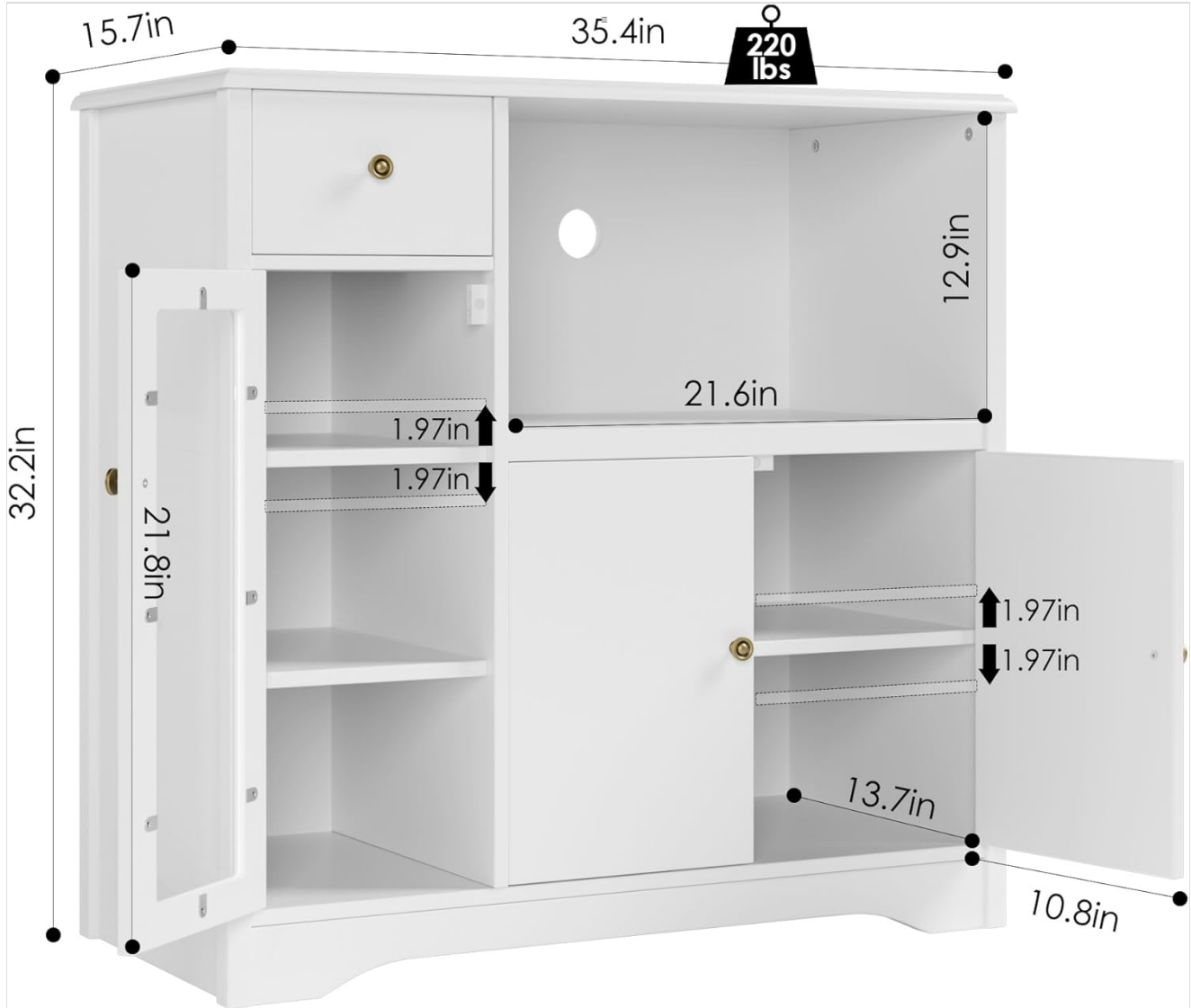
Figure 4.1: Cabinet Dimensions and Load Capacity
