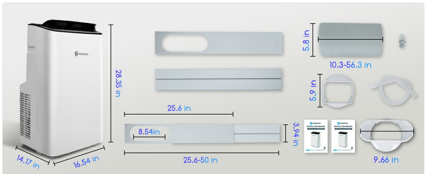
Figure 3.1: Included components and their approximate dimensions.
