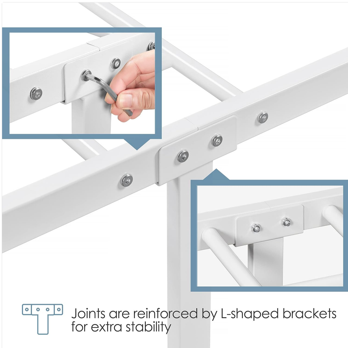
Figure 2: Joints are reinforced by L-shaped brackets for extra stability.
