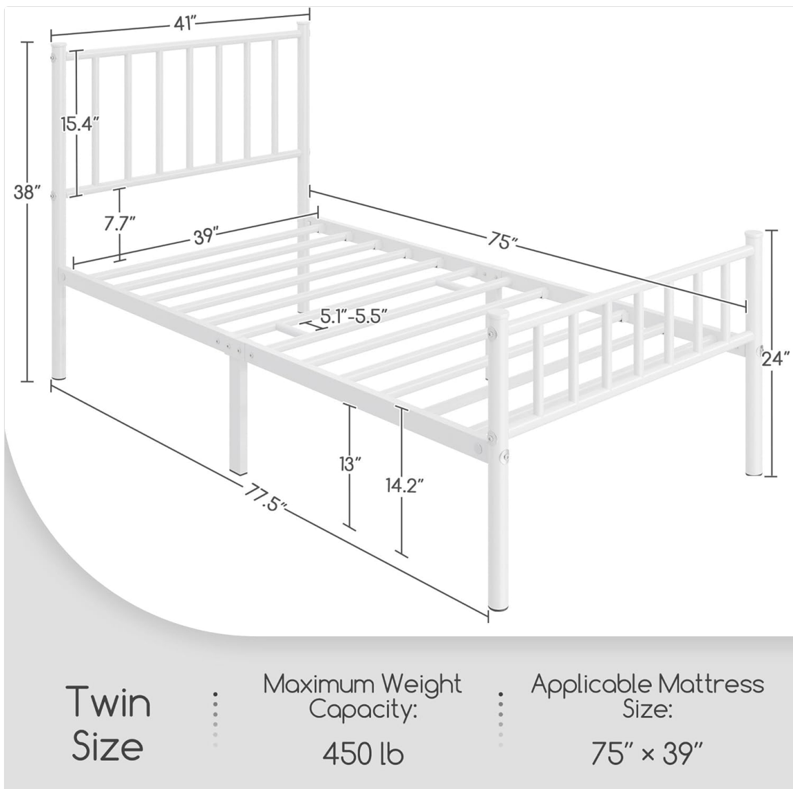
Figure 7: Detailed dimensions and specifications of the twin bed frame.
