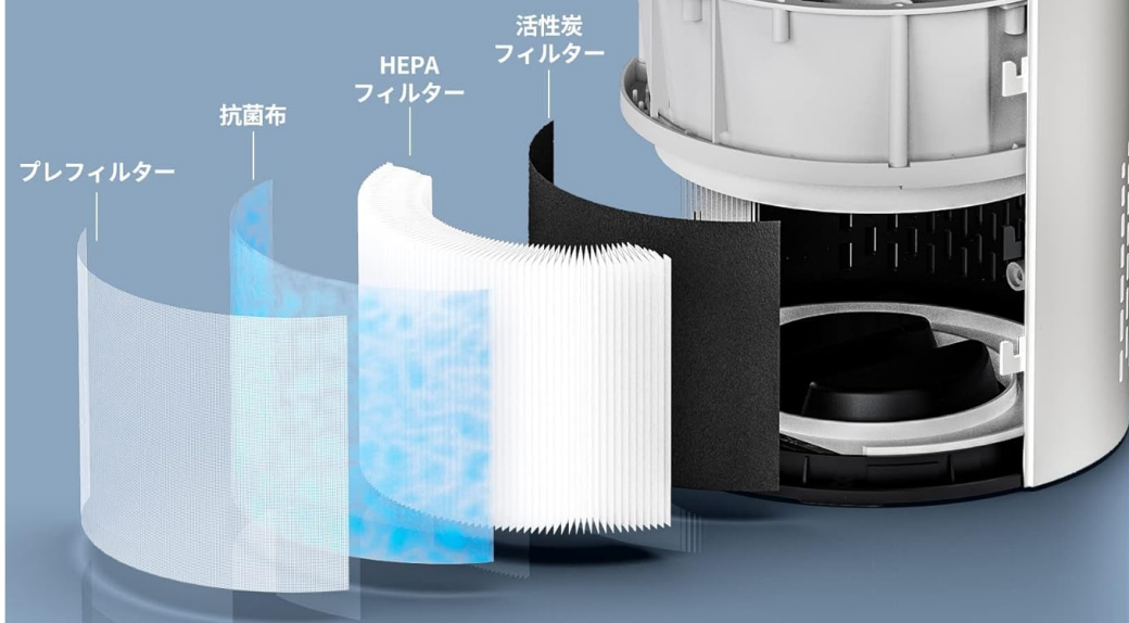
Image: An exploded view of the air purifier's multi-layer filter, showing the pre-filter, activated carbon filter, and HEPA filter components.
