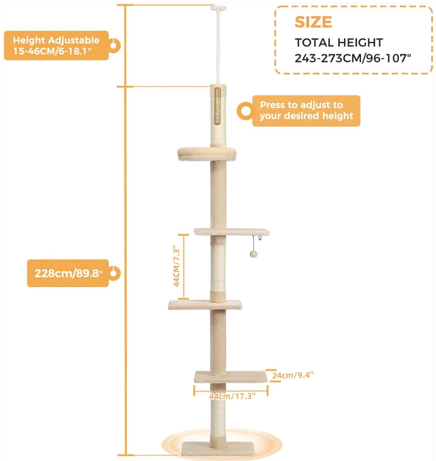
Figure 1: Product dimensions and adjustable height mechanism. The total height ranges from 95 to 107 inches (243-273 cm).
