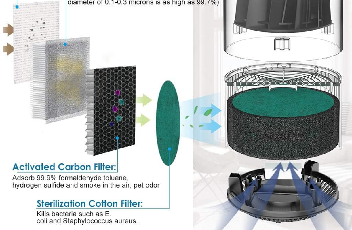
Image: Detailed diagram illustrating the four stages of filtration: Pre-Filter, HEPA Filter, Activated Carbon Filter, and Sterilization Cotton Filter, along with the air flow path.
