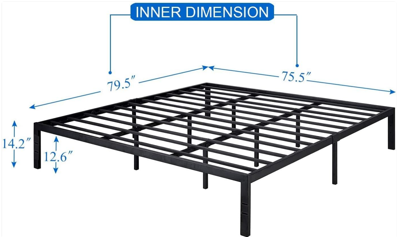
Image: Dimensional diagram of the King size bed frame.
