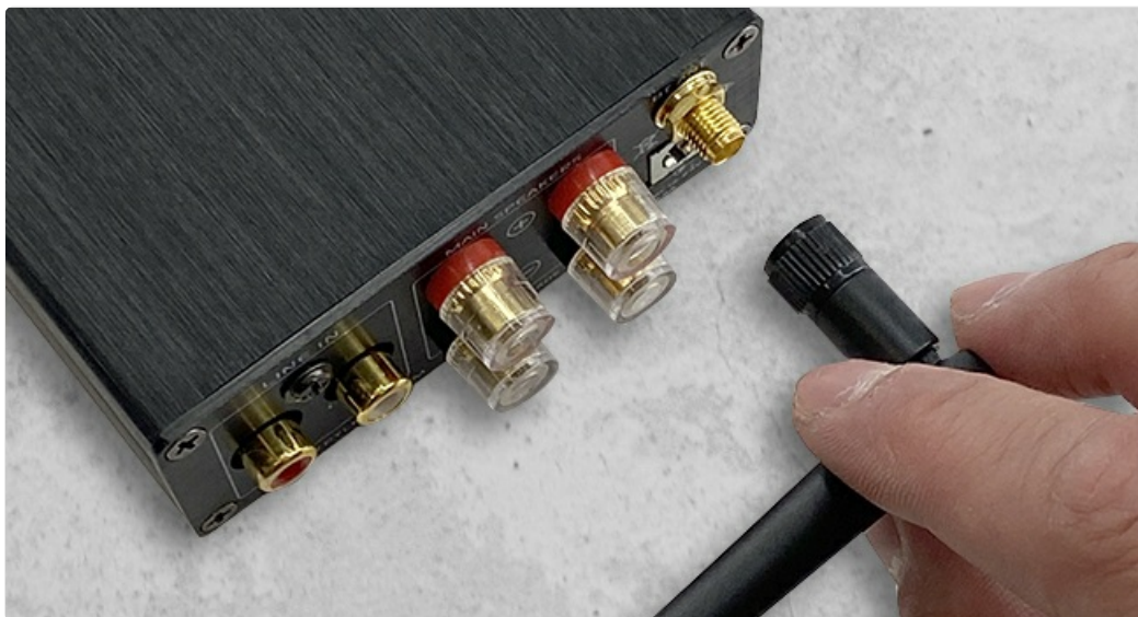
Figure 5.3: A hand attaching the Bluetooth antenna to the designated port on the rear of the amplifier.
