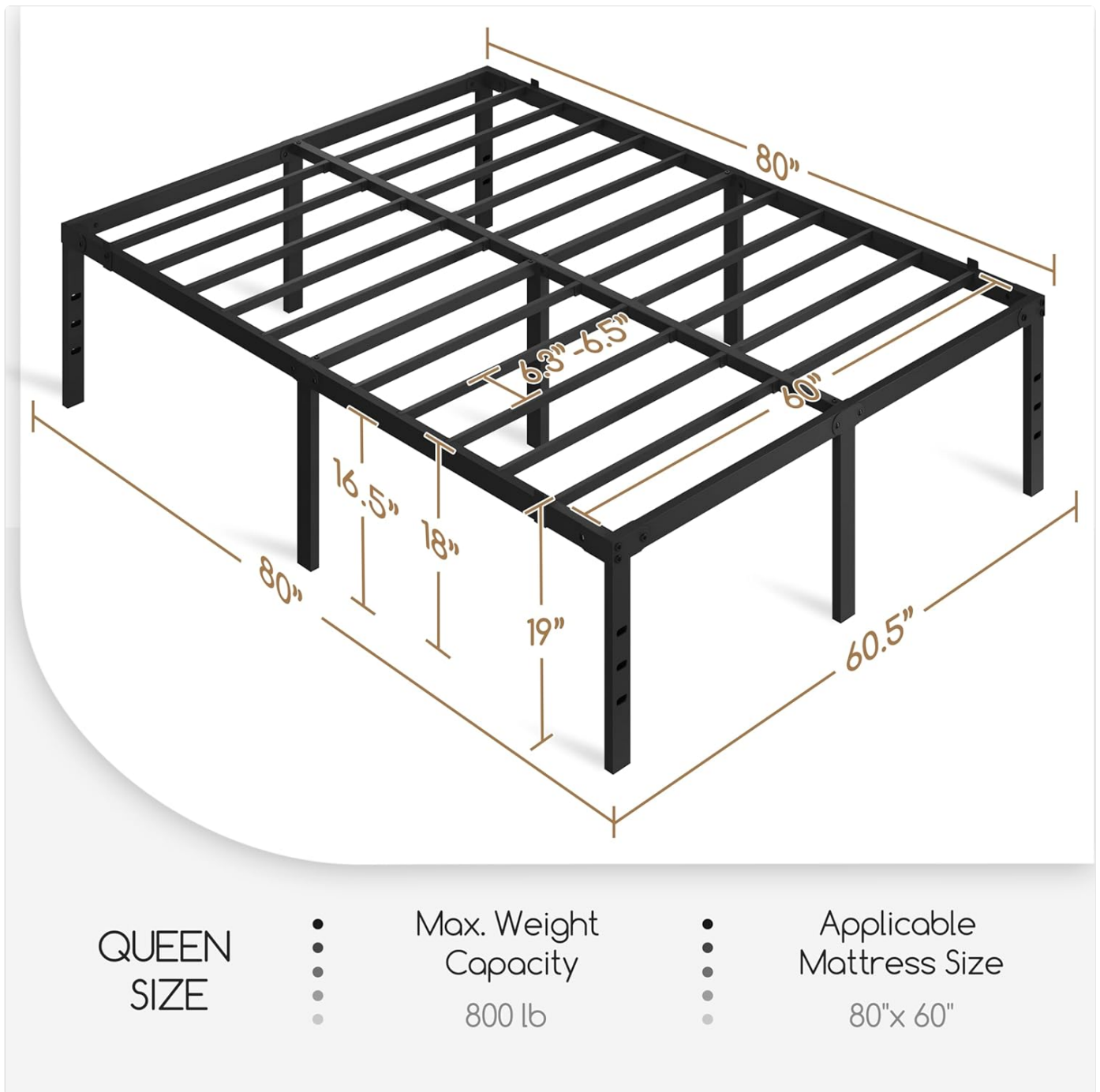
Image: A comprehensive diagram displaying the key dimensions of the Yaheetech Queen Bed Frame, including length, width, height, and under-bed clearance.
