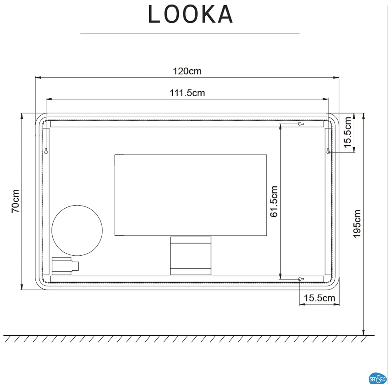
Figure 3: Dimensional drawing of the SENSEA LOOKA LED Bathroom Mirror (120 cm x 70 cm).
