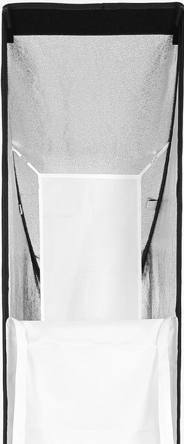
Image 3.2: Close-up of the internal double diffuser and the Bowens mount adapter ring.
