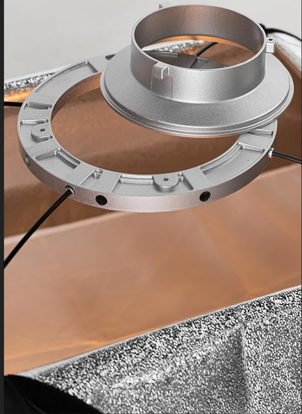
Image 3.2: Close-up of the internal double diffuser and the Bowens mount adapter ring.
