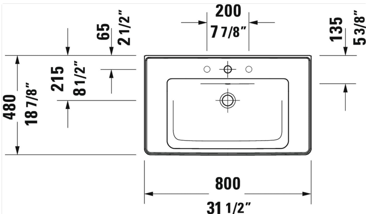
Figure 3: Top view of the Duravit D-Neo Vanity Sink with imperial dimensions, indicating width, depth, and basin measurements.
