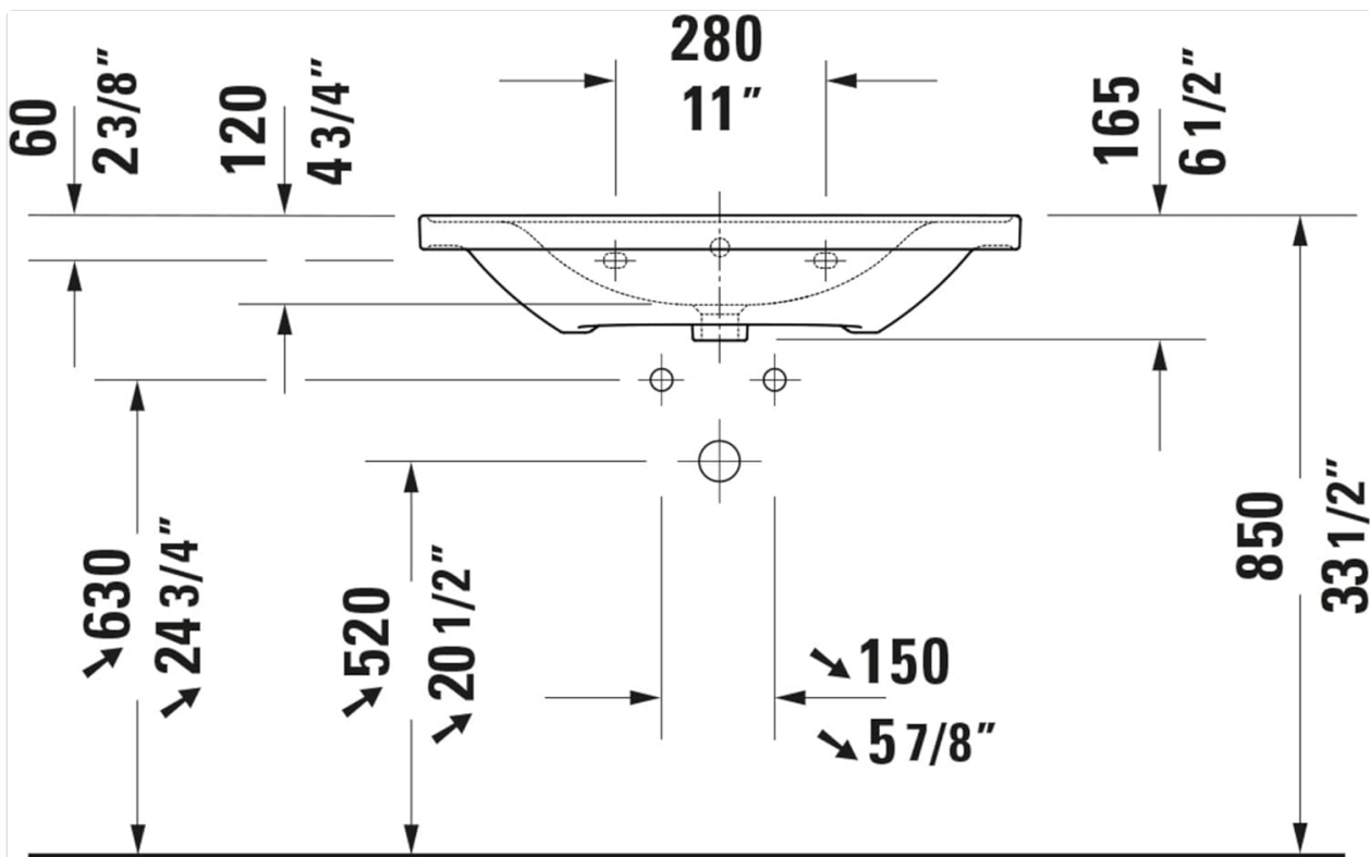
Figure 2: Side view of the Duravit D-Neo Vanity Sink with imperial dimensions, showing height, depth, and faucet hole placement.
