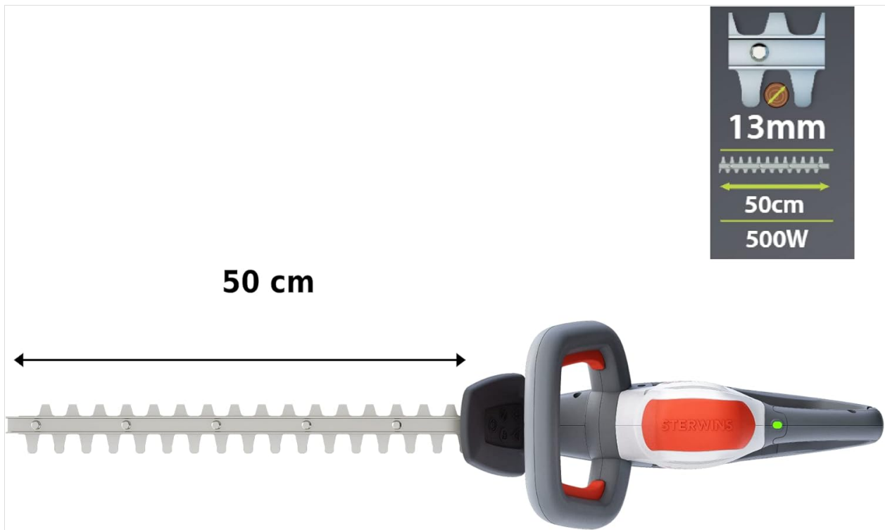
Image 3: Illustration of the 50 cm blade length and 13mm cutting capacity.
