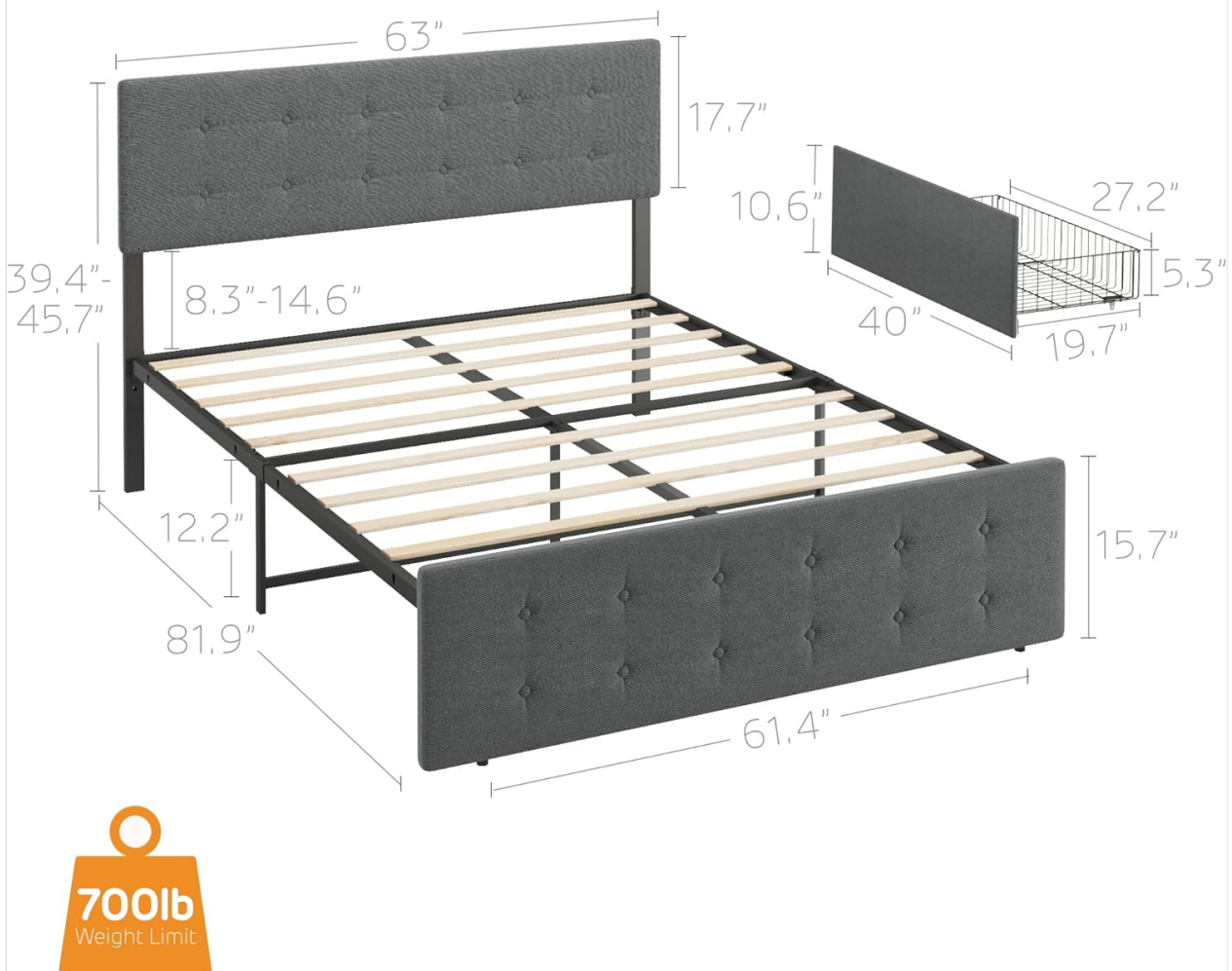
Figure 3.1: Product Dimensions and Components Overview.
