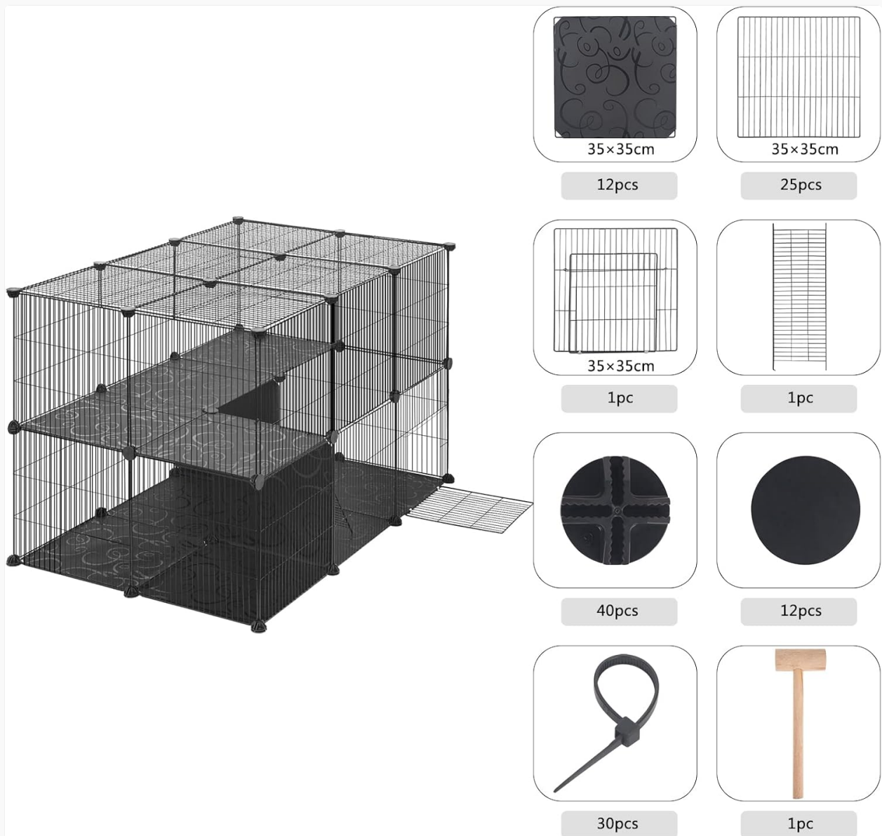
Image: All included components for assembly.
