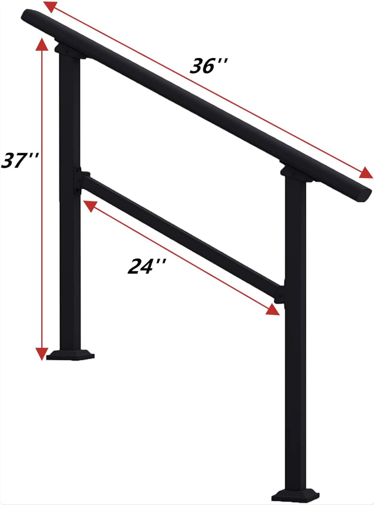
Image: Dimensional drawing of the handrail, indicating key measurements.
