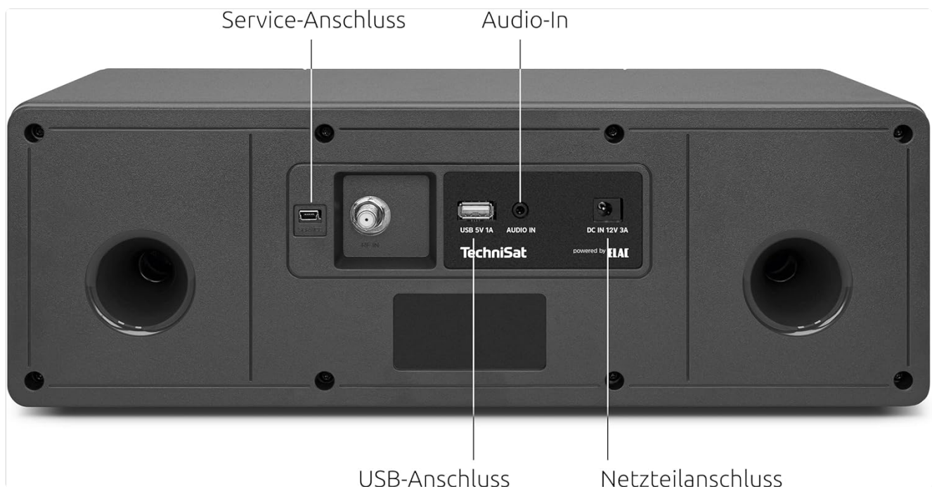
Figure 2: Rear Connections. This image highlights the rear panel connections, including the Service Port, Audio-In, USB Port, and Power Supply Connection (DC IN 12V 3A).
