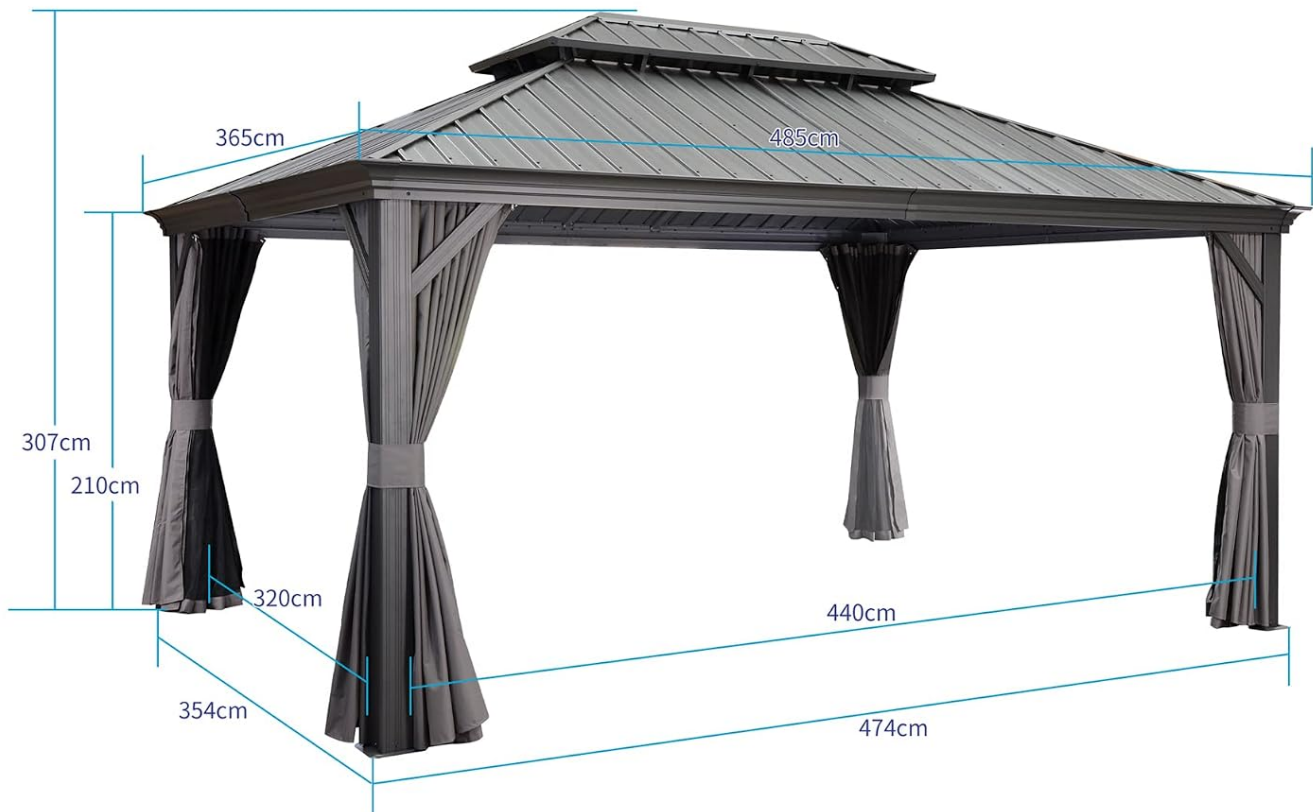
Image 4.1: Detailed dimensions of the gazebo, including height and footprint.
