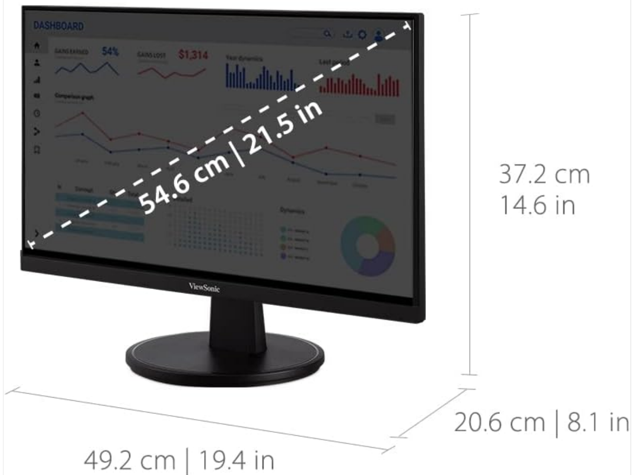
Figure 6: Physical dimensions of the VS2247-MH monitor.
