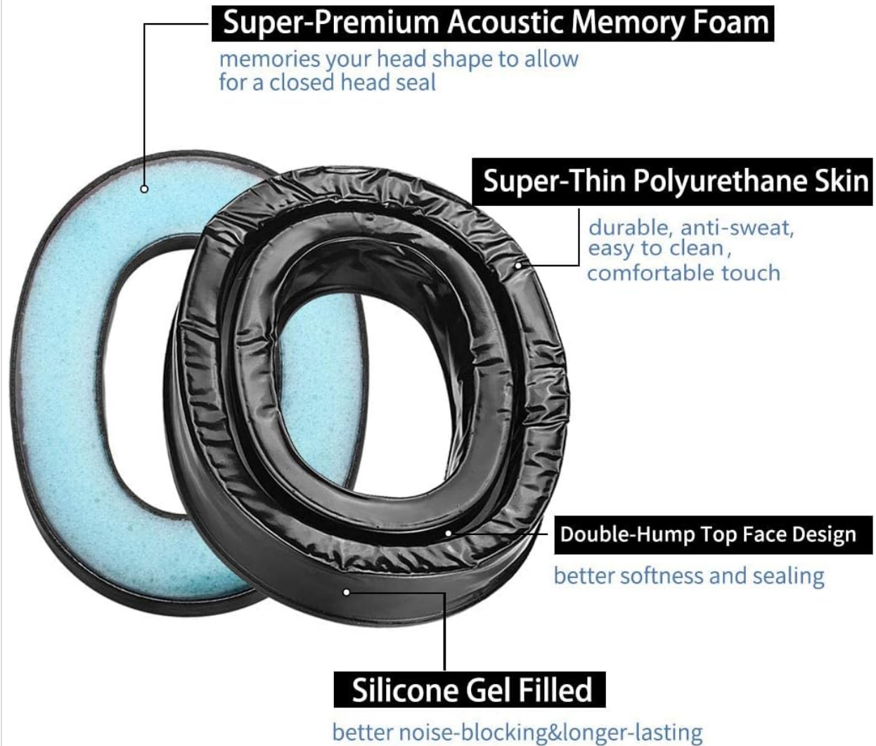
Image 4.3: Detailed construction of GEP01 Memory Foam Gel Ear Pads.
