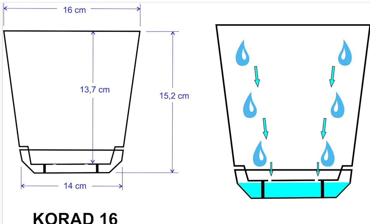
Image 2.1: Technical diagram illustrating the dimensions and the integrated drainage system of the KORAD flower pot.
