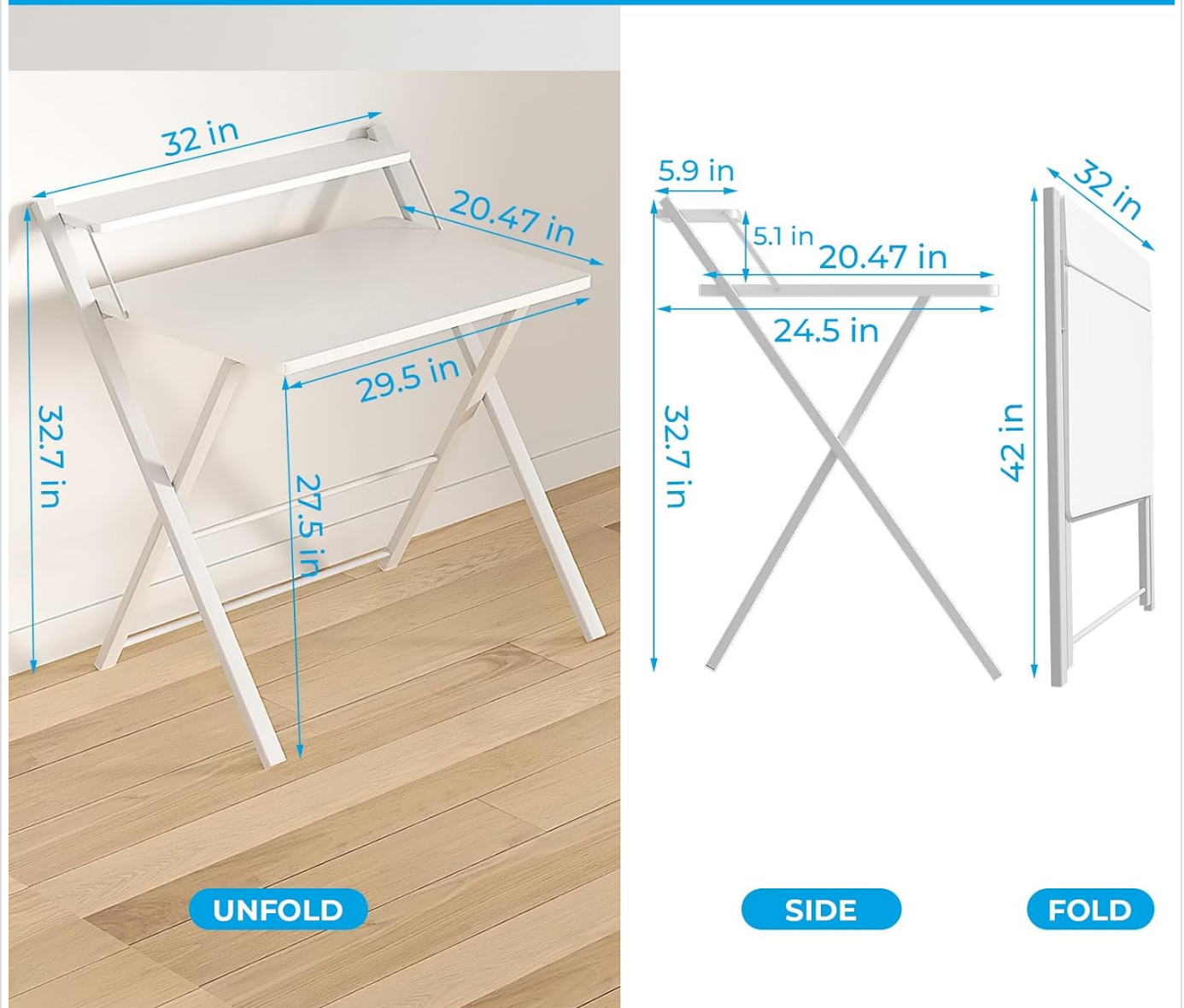
Figure 9: Detailed dimensions of the desk in various states (unfolded, side view, and folded).
