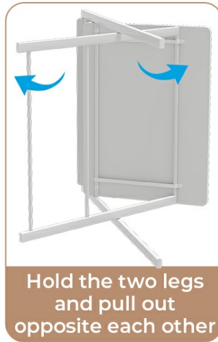
Figure 4: Detailed steps for unfolding the desk, showing the movement of the legs and tabletop.
