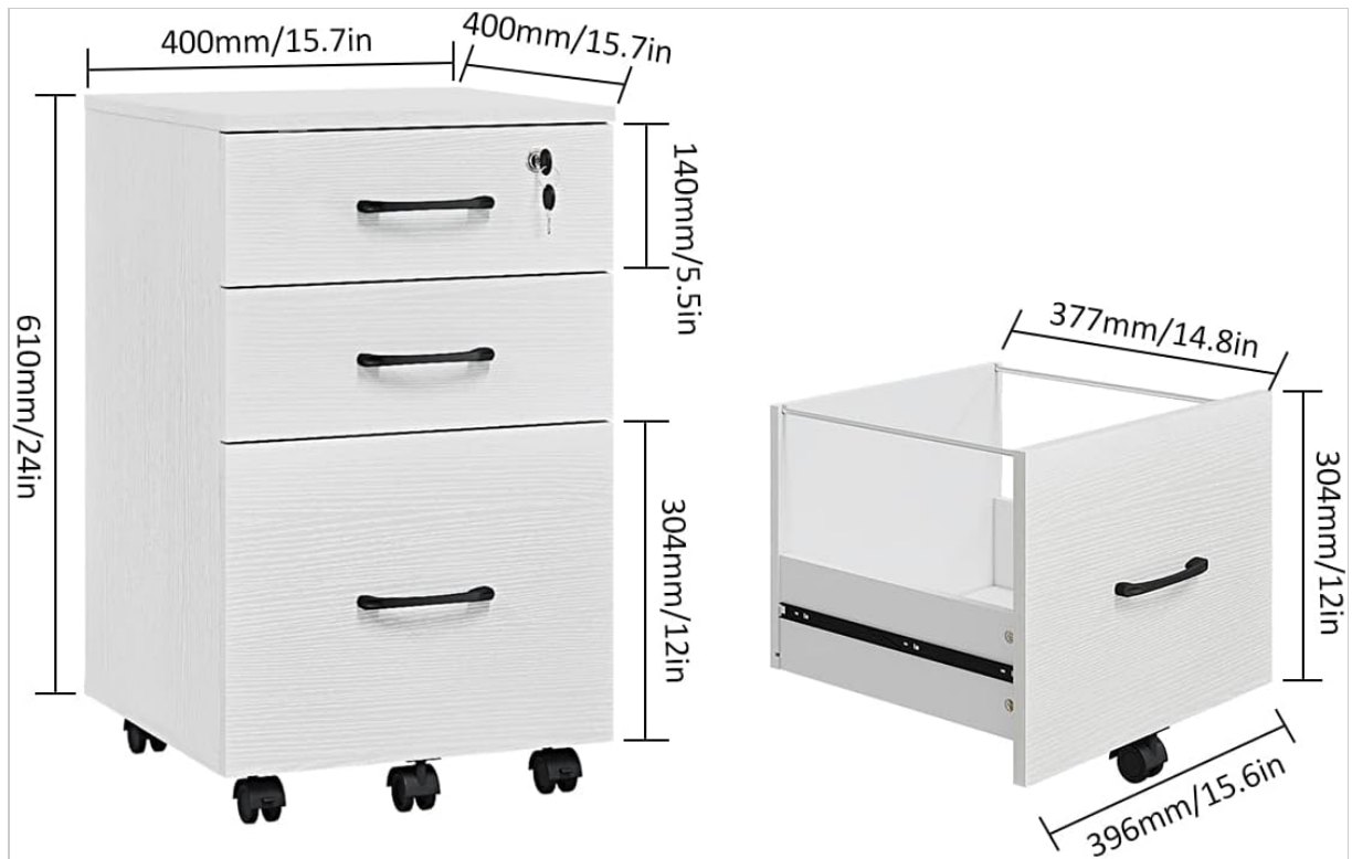
Image 4: Detailed dimensions of the Panana 3-Drawer Mobile File Cabinet, showing height, width, and depth in both millimeters and inches.
