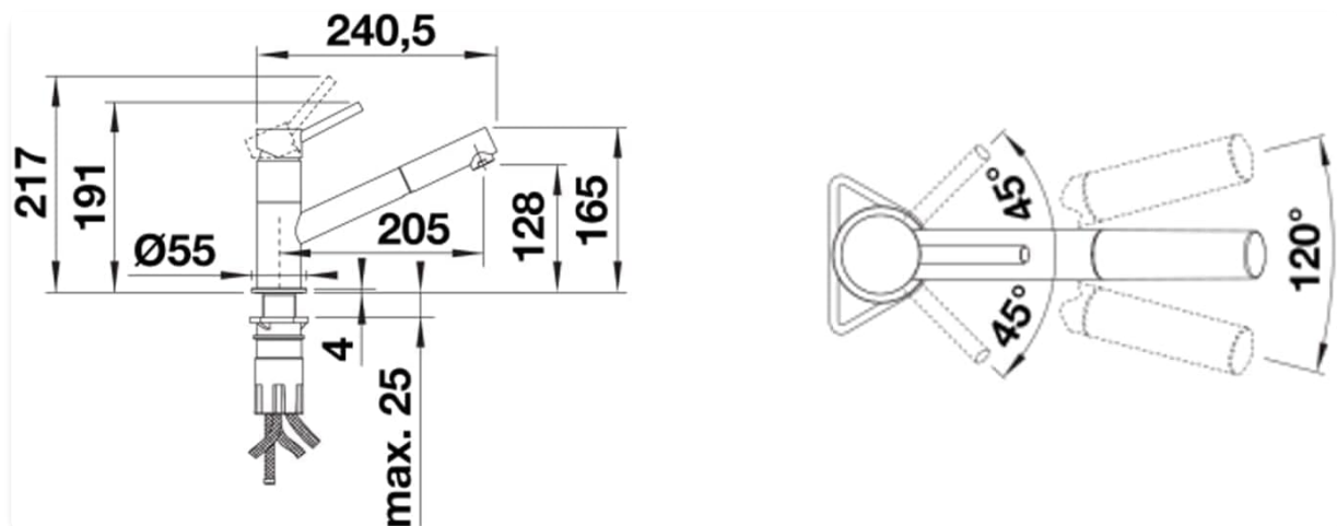
Figure 2: Technical drawing showing the dimensions and installation details of the BLANCO Kano-S faucet. This diagram illustrates the spout height, depth, and overall dimensions for installation planning.
