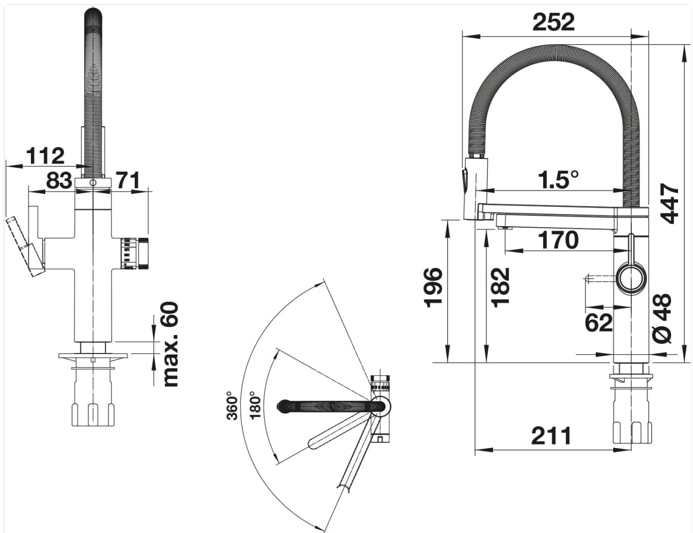
Figure 2: Technical drawing showing the dimensions and installation requirements for the faucet.
