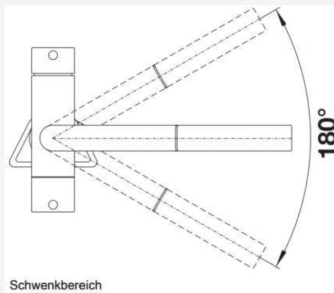
Image: Top-down diagram illustrating the 180-degree swivel range of the faucet spout.
