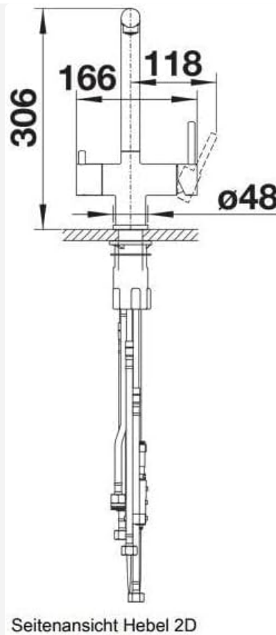
Image: Side view diagram of the faucet with key dimensions (height 306mm, spout reach 166mm) and lever position.
