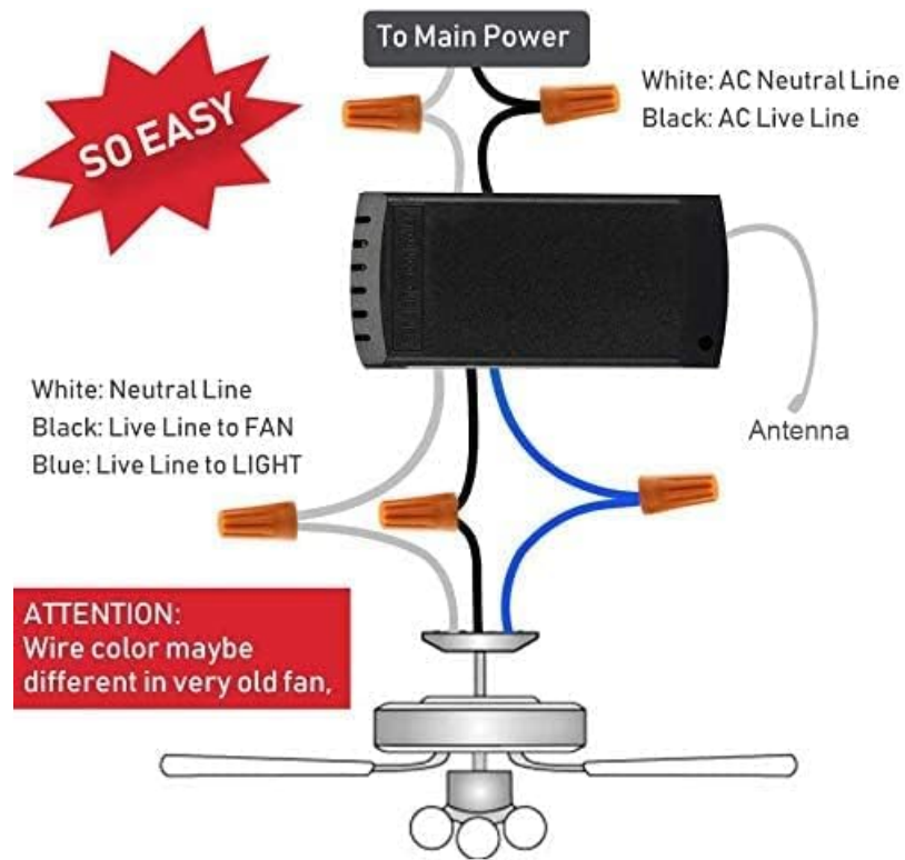
Image: Wiring diagram showing connections from main power to the receiver (White: AC Neutral Line, Black: AC Live Line) and from the receiver to the fan (Black: Live Line to FAN, Blue: Live Line to LIGHT).
